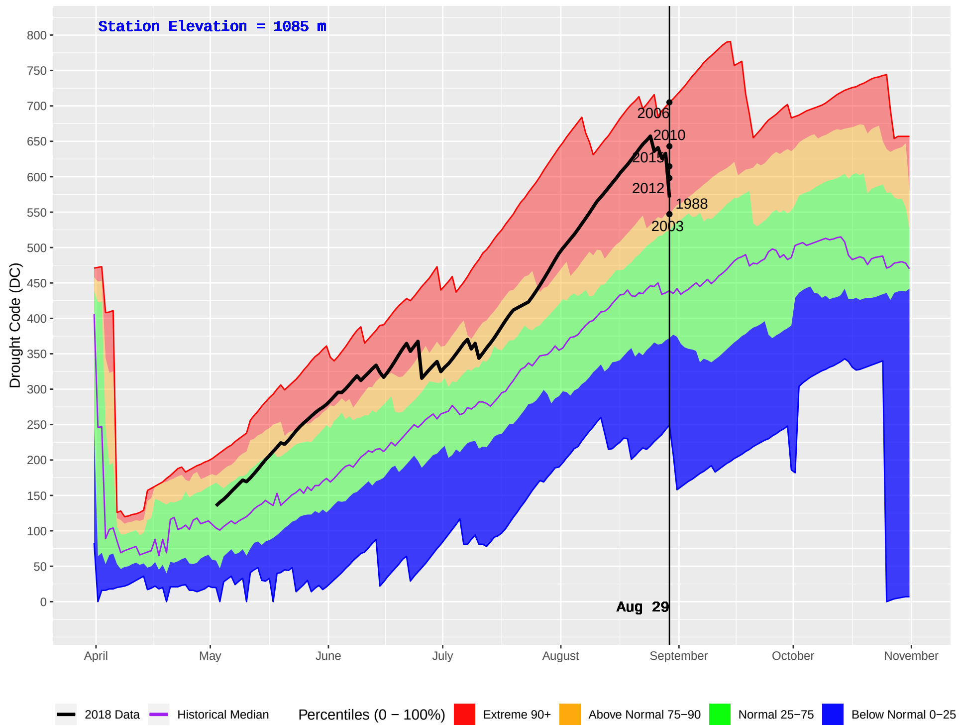
TAUTRI (206) : Historical (1970–2016) and Current (2018) Daily Drought Code (DC)
